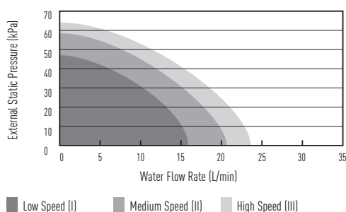
Hydraulic Pump Performance. 9 kW single phase
