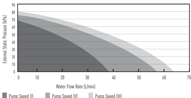
Hydraulic Pump Performance. MDC 12 to MDC 16 single phase and all MDC three phase
