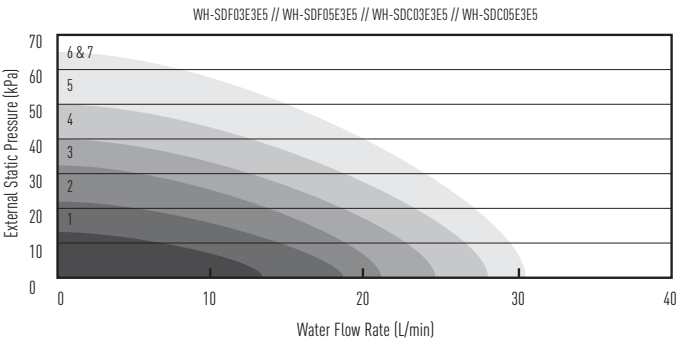
Hydraulic Pump Performance. Constant Pressure Head Difference (Δp-c). 3 and 5kW
