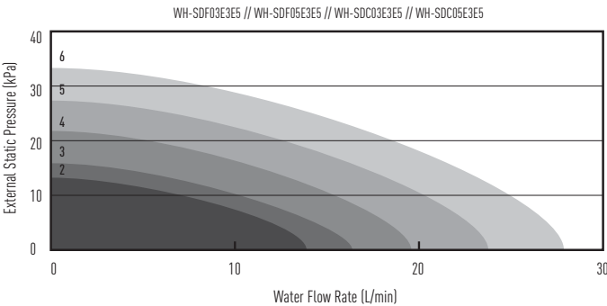
Hydraulic Pump Performance. Variable Pressure Head Difference (Δp-v). 3 and 5kW
